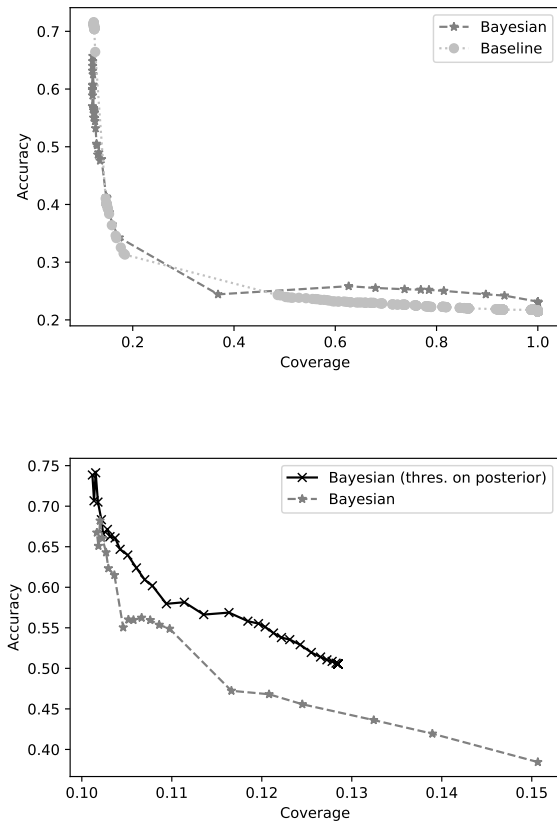
Figure 2: Accuracy versus coverage. (Top) Baseline and Bayesian model. (Bottom) Bayesian model with and without threshold on the posterior probability of the parameters.
